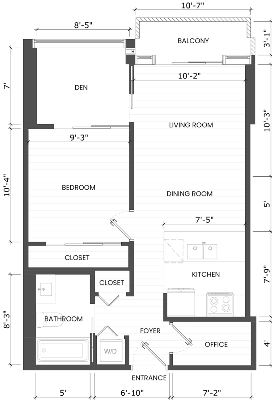
MAIN FLOOR PLAN Ceiling Height: 8'-0"
